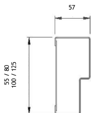
Single rabbet frame
