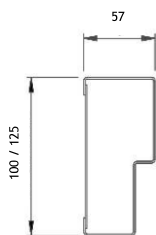
Single rabbet frame
