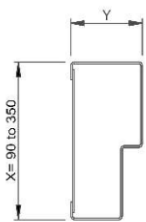
Single rabbet frame
